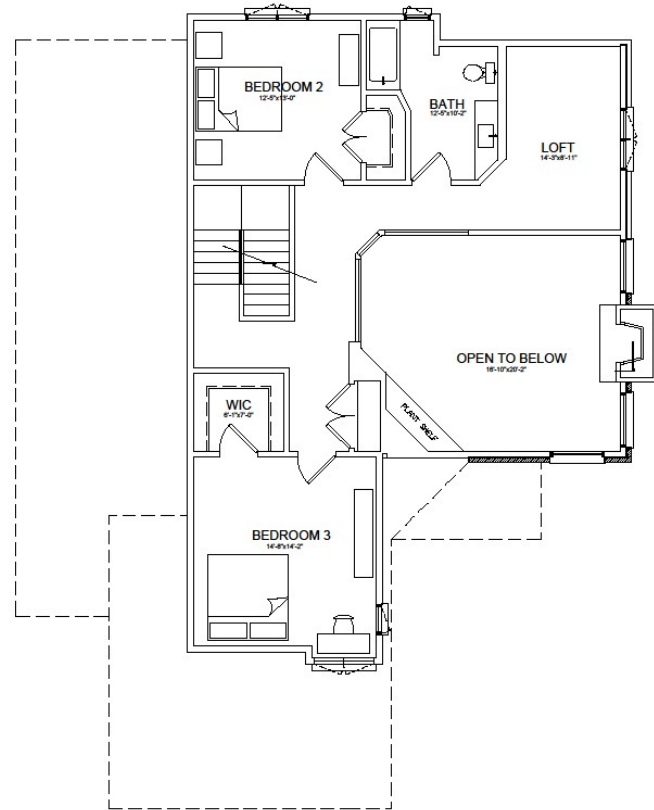
GLASTONBURY II SECOND FLOOR PLAN
