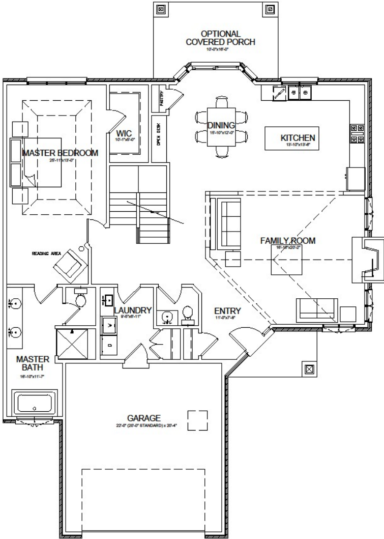
GLASTONBURY II FIRST FLOOR PLAN
